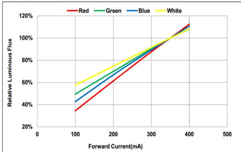
Fig 3. IF Vs. Relative Intensity (亮度与电流关系), Ta = 25°C
