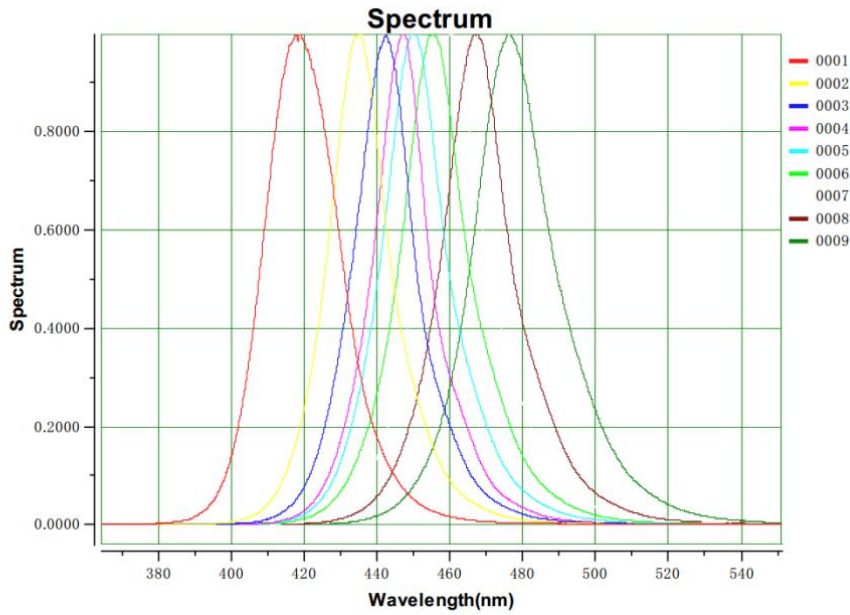
Fig 2. Radiation Diagram (发光角度), Ta = 25°C, RH60%
